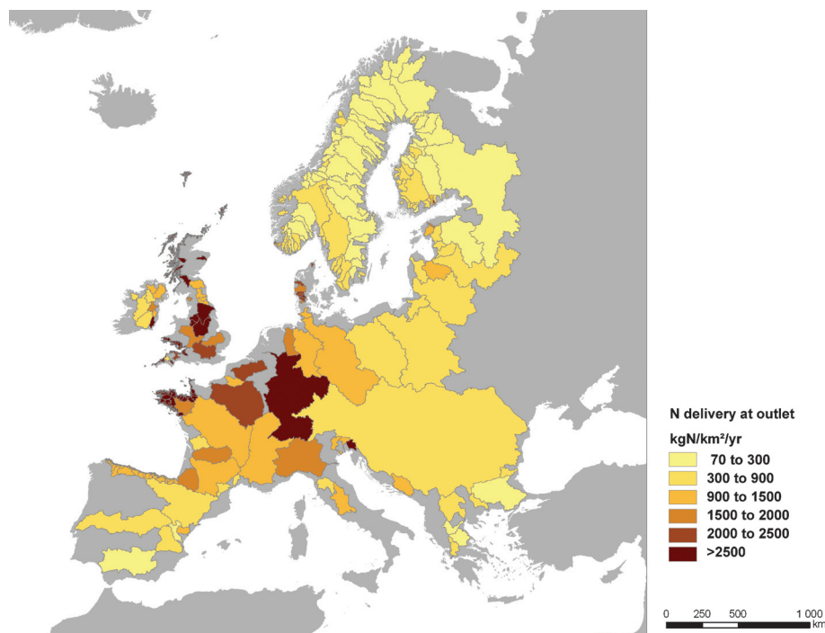
Figure 13.6 Available observed data on N delivery by European watersheds. Data from Humborg et al. (2003, 2006, 2008); Radach and Pätzsch (2007); Lancelot et al. (1991); Billen et al. (2009a, b); Neal and Davies (2003); Meybeck et al. (1988); Ludwig et al. (2009); Cociasu et al. (1996); Johnes and Butterfield (2002); OSPAR (2002); REGINE (2010). See online supplementary material (Section 13.7) for original data.
