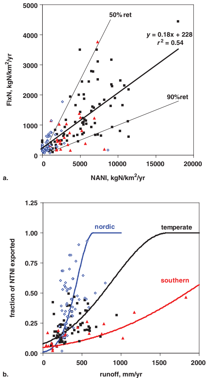
Figure 13.8 (a) Specific N flux delivered at the outlet of European watersheds as a function of the net anthropogenic nitrogen inputs (NANI). The heavy line represents the regression across all points. The lighter lines represent N retention of 50% and 90% of NANI. (b) Fraction of NTNI delivered at the outlet as a function of runoff for Scandinavian (◇), temperate (■) and Mediterranean (▲) watersheds. The line represents the best fit of the sigmoid relationship proposed by Billen et al. (2010): \text{fraction NTNI exported} = \exp(-(Q-Q_m)^2/Q_s^2) , where Q is the mean specific runoff (mm/yr) of each watershed and Q_m and Q_s are climate-specific parameters.
